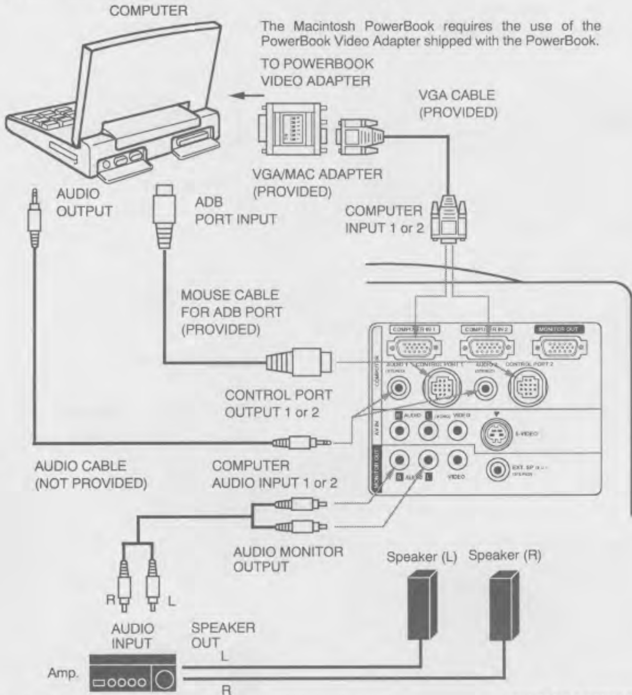
VGA/MAC ADAPTER
